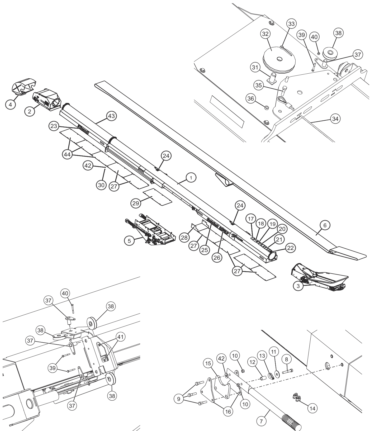
Winch Cable Sheave Ass'y
